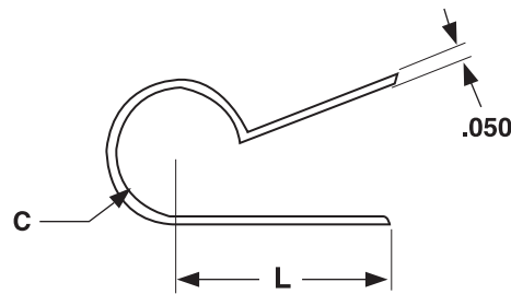
NYLON HEAVY DUTY CABLE CLAMPS—1/2" WIDE CONTACT AREA
