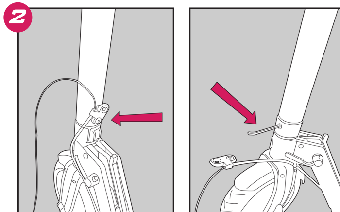
STEP 2: Remove the screws near the fold
