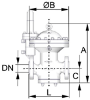
Dimensional Sketch (Example) HON R100NG
