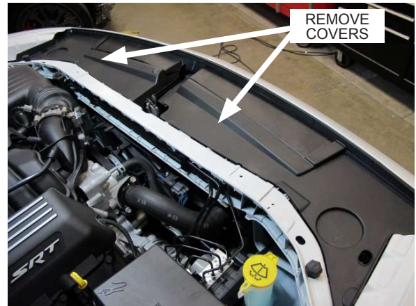
Fig. 2-a: Remove covers
