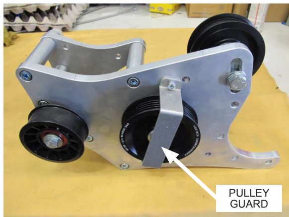
Fig. 5-a: Remove pulley guard
