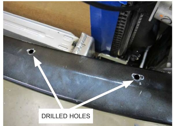
Fig. 6-v: Drill 2x holes using 6" length drill bit
