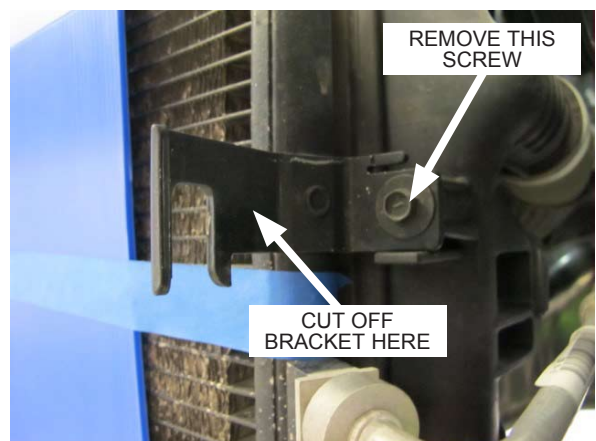
Fig. 6-f: Remove aluminum bracket and screw
