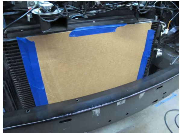
Fig. 6-e: Cover A/C condenser with cardboard
