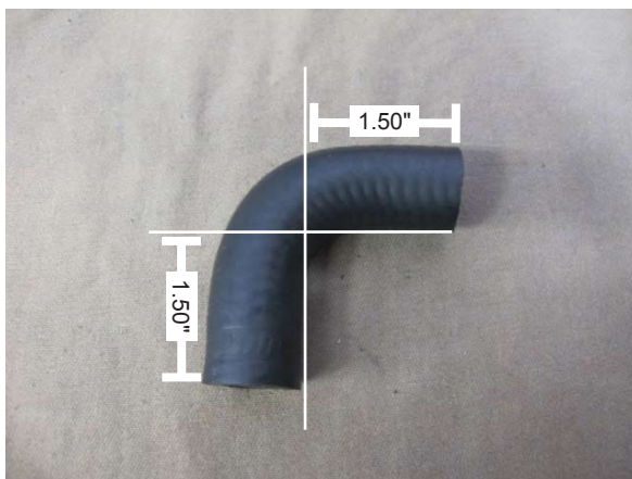
Fig. 8-o: Modify 1/2" x 90° coolant elbow as shown
