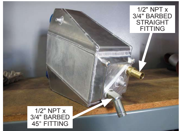
Fig. 6-d: Install fittings to air/water cooler
