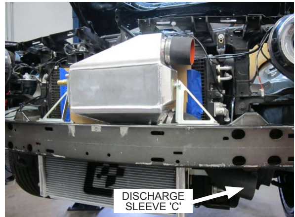
Fig. 6-y: Install air/water cooler
