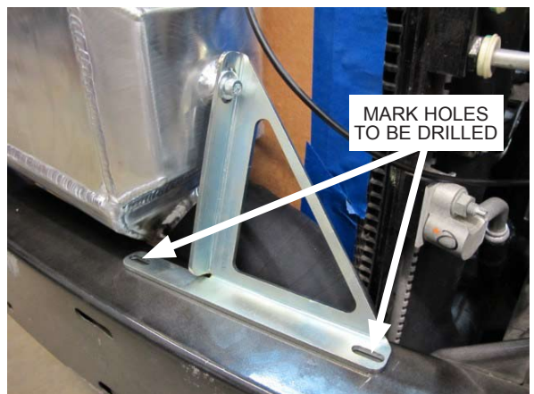
Fig. 6-u: Use driver side air/water cooler support bracket as drill template
