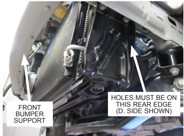
Fig. 4-h: Reinstall lower radiator support
