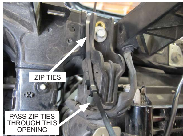
Fig. 2-o: Zip tie radiator to core support
