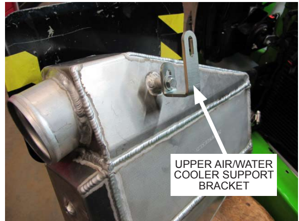
Fig. 6-q: Install upper air/water cooler support bracket
