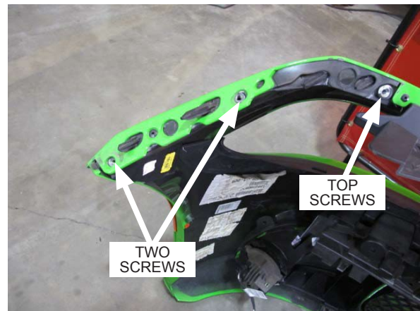
Fig. 2-h: Remove screws (Bumper removed for clarity)
