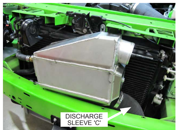
Fig. 6-x: Loosely install upper air/water cooler support bracket and air/water cooler
