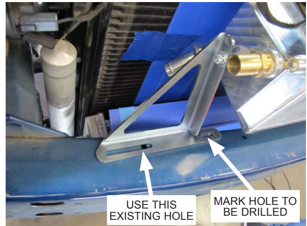
Fig. 6-s: Mark the holes to be drilled on the passenger side of the front bumper support
