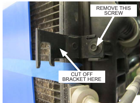
Fig. 6-g: Remove aluminum bracket and screw
