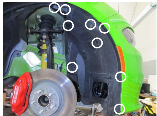
Fig. 2-c: Remove fender liner fasteners
