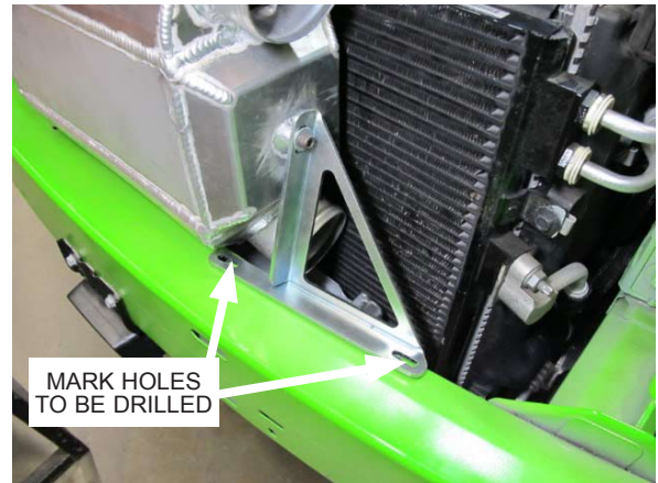
Fig. 6-t: Mark the two holes to be drilled on the driver side of the front bumper support
