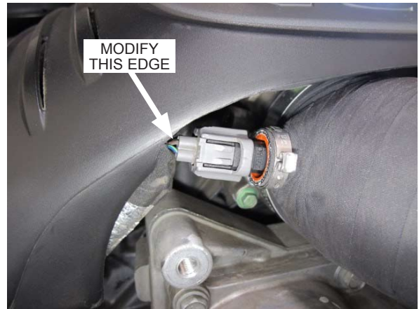
Fig. 9-b: Modify driver side engine cover
