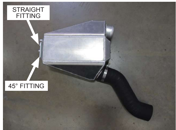
Fig. 6-w: Install discharge sleeve 'C' to the air/water cooler as shown
