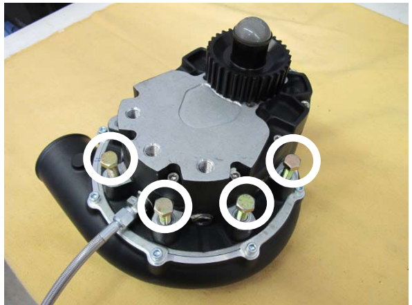
Fig. 7-b: Lubricate supercharger mounting boss threads
