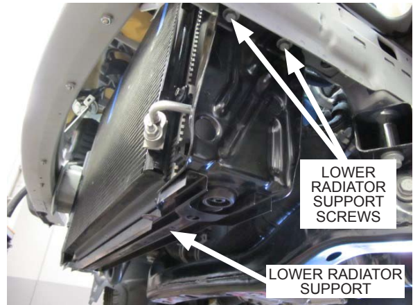
Fig. 2-p: Remove lower radiator support hardware
