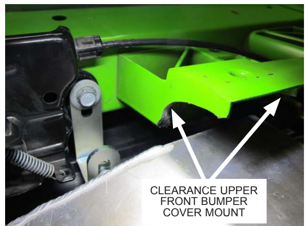
Fig. 6-r: Clearance the front bumper cover mount
