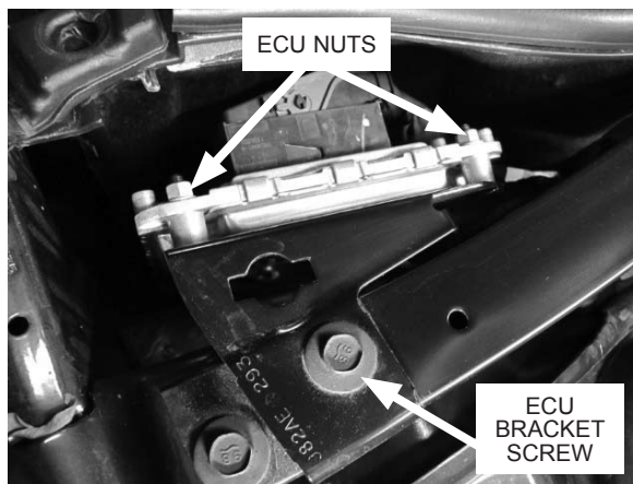
Fig. 1-e: Remove ECU nuts and remove cross bar screws
