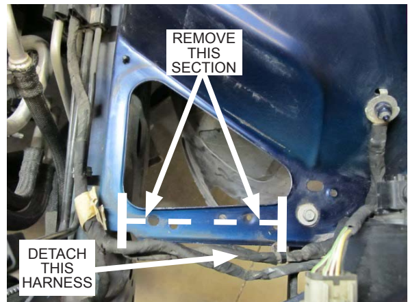
Fig. 6-e: Modify driver side inner wheel well as shown
