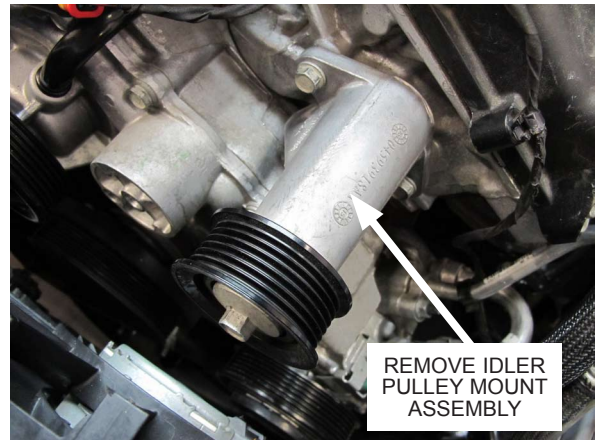
Fig. 2-s: Remove idler pulley mount assembly
