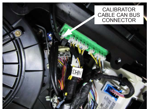
Fig. 10-f: Connect CAN bus connector
