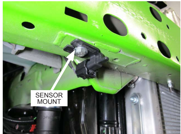
Fig. 6-ak: Reinstall ambient air temperature sensor as shown
