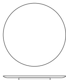
T119-6 60" Diameter Round Top 60"Dia x 1.75"H
